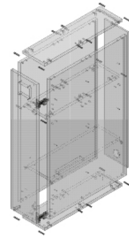
Exploded view
