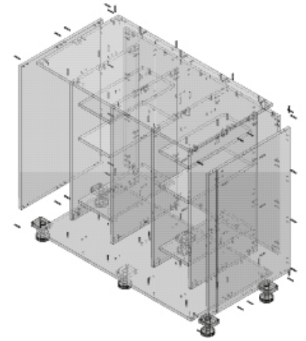
Exploded view
