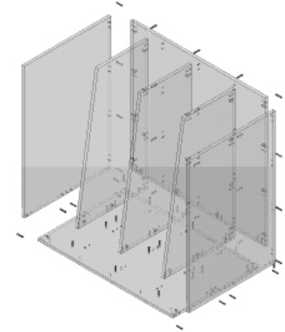
Exploded view
