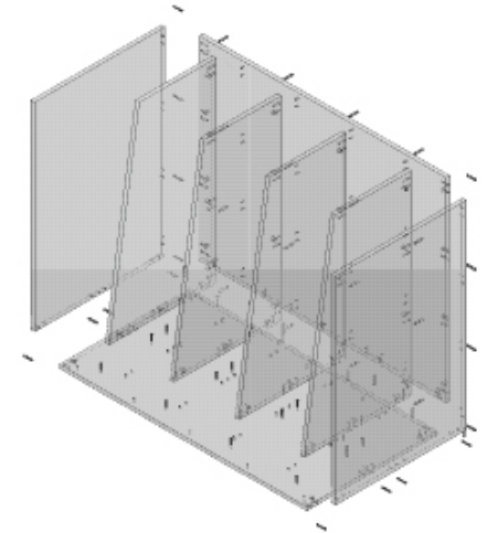
Exploded view
